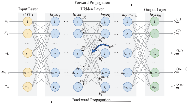
Figure 1: The architecture of MLP.
