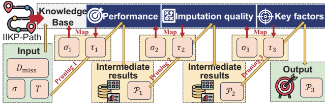
Figure 21: The pruning recommendation method workflow.
