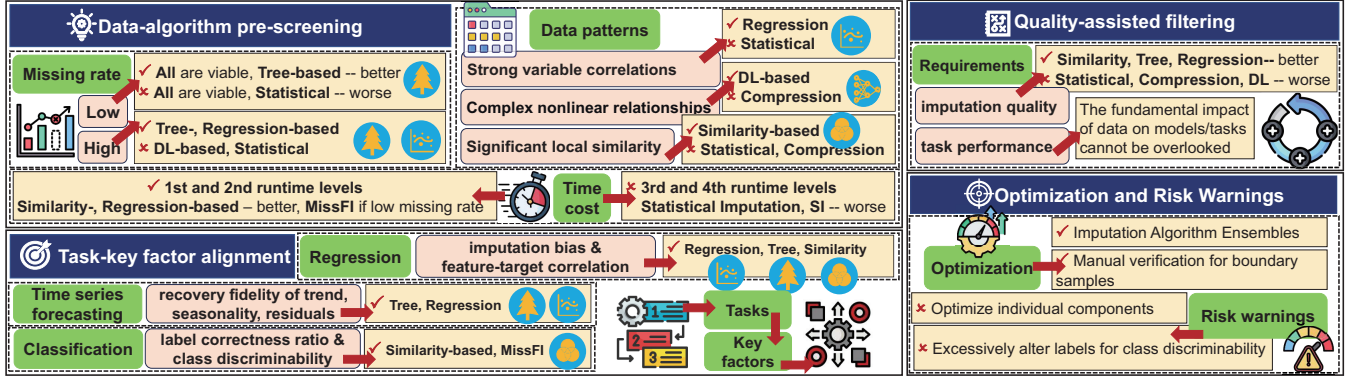
Figure 20: The workflow of basic recommendations.
