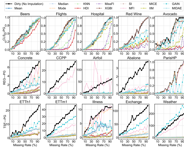
Figure 9: Downstream performance of three tasks.
