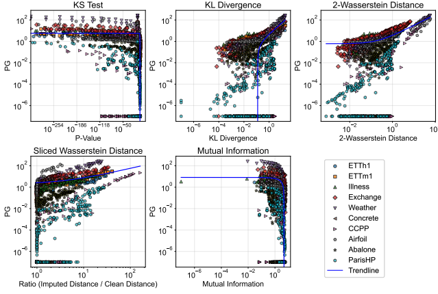
Figure 11: The distribution of quality and performance.
