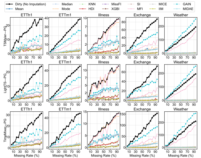
Figure 10: Downstream performance of three models.
