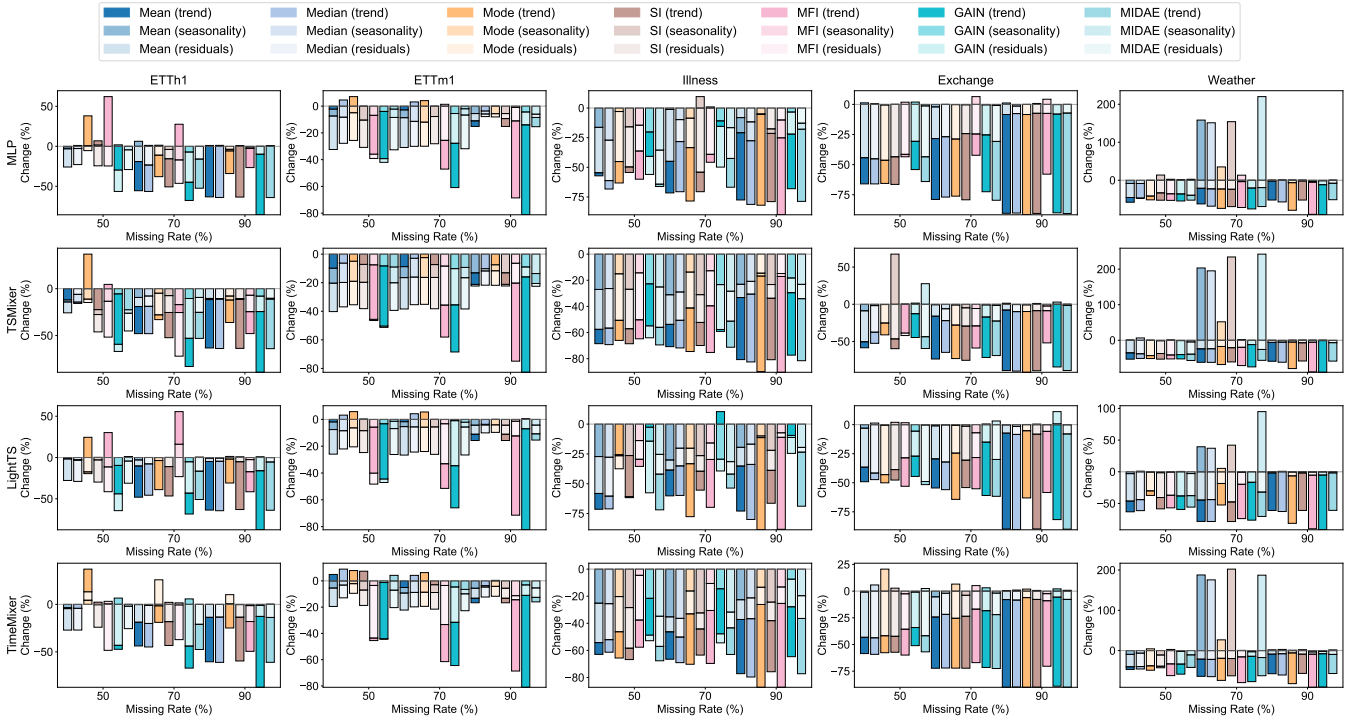
Figure 19: The percentage change in performance from pre- to post- replacement.
