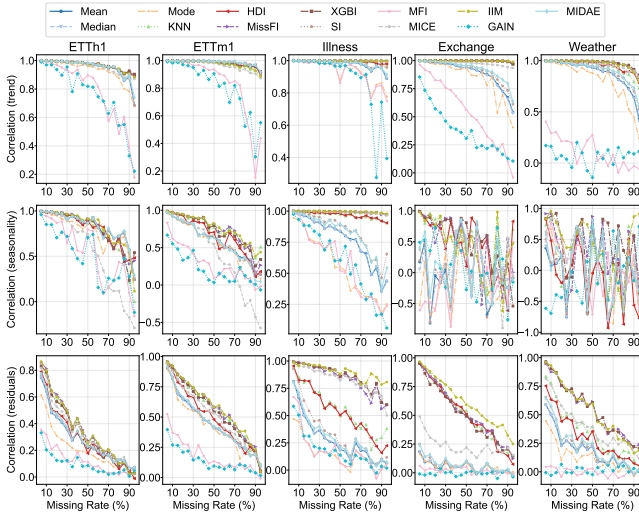
Figure 18: Correlation coefficient in time series forecasting.
